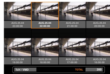
<Thumbnail window>
