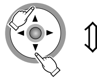
<List window>
